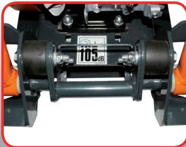
Anti-Vibration Handle Mounts & Lifting Point
